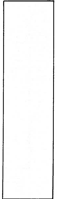
i tetromino
